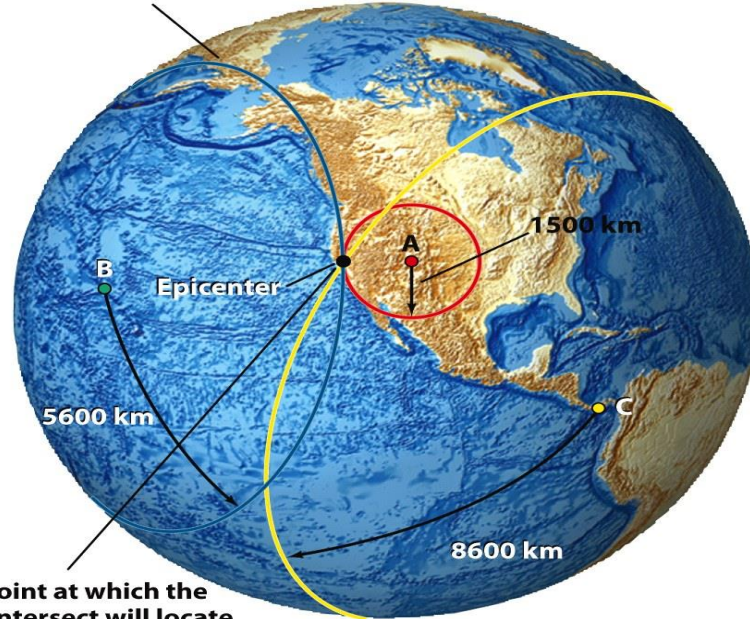
Figure 13.9 part 3 Understanding Earth , Sixth Edition © 2010 W. H. Freeman and Company
