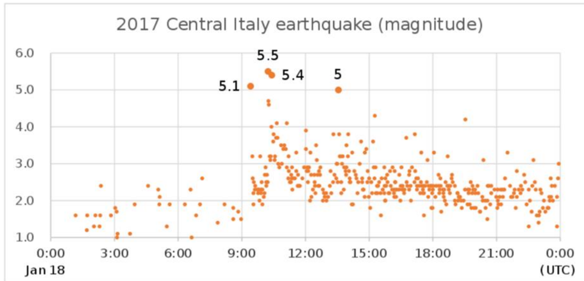
Magnitude of January 2017 earthquakes
